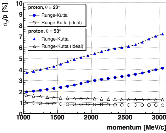
Fig. 34. Simulated momentum resolution for protons with realistic errors (GARFIELD errors multiplied by 4) shown for the Runge-Kutta method (full symbols) and compared to the case without applying any detector resolution (“Runge-Kutta ideal”; open symbols) for 2 different polar angles.
