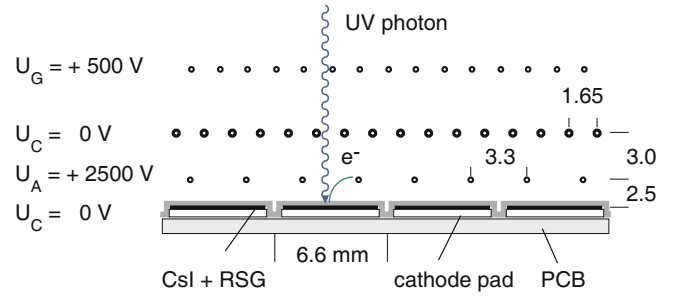
Fig. 5. Schematic cross-section of the MWPC part of the photon detector. The different wire planes comprise a gate, a cathode and an anode. All distances are given in millimeter. The asymmetric field configuration increases the charge fraction induced onto the pads to about 70%. The entrance window is not shown.
