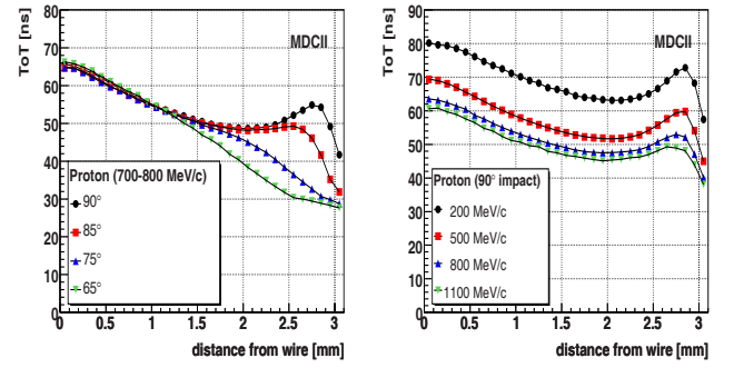
Fig. 13. Left: dependence of ToT on the distance from wire to particle track for 0.7–0.8 GeV/c protons at 4 impact angles. Right: same for protons with a average impact angle of 90° and different momenta (shown for MDCII).
