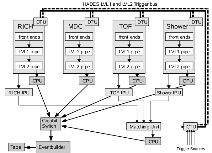
Fig. 28. Block diagram of the trigger distribution and data acquisition system. Triggers are sampled by the central trigger unit (CTU) and transported via the trigger bus to the Detector Trigger Units (DTUs). The data is stored in the LVL1 pipe. At the same time pattern recognition algorithms are performed in Image Processing Units (IPUs), a Matching Unit (MU) finally combines this information. After a positive decision, the data is read out via the VME CPUs and sent to the event builder.
