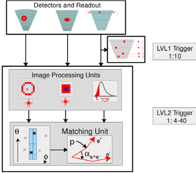
Fig. 29. Overview of the reduction capabilities of the complete HADES trigger system. The first-level trigger (LVL1) is generated via charge multiplicity measurement with a certain admixture of minimum bias and calibration triggers. The second-level trigger is searching for electron hit candidates in the RICH, Pre-Shower and TOF detectors which are correlated using the matching unit. The reduction factor of the LVL2 algorithm is 4–40, depending on the reaction under consideration.
