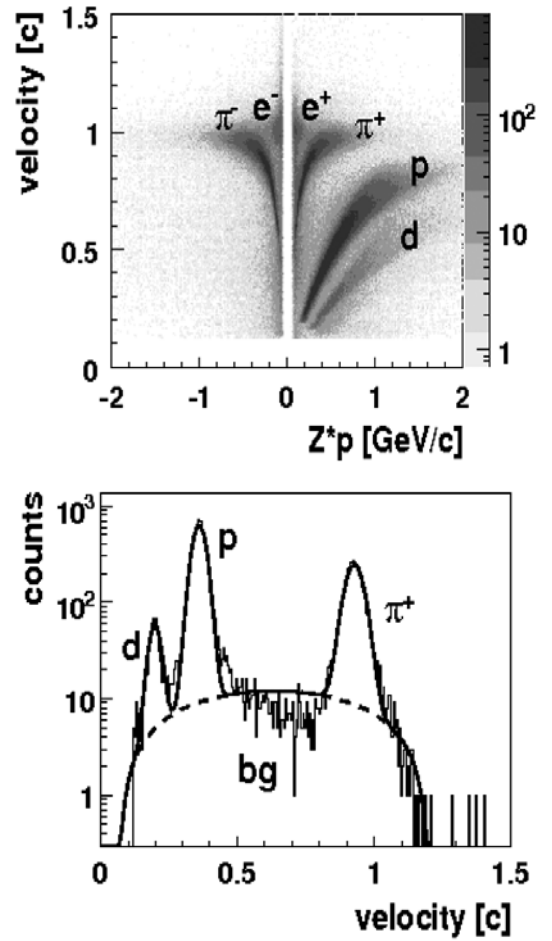
Fig. 39. Top: velocity versus Zp of charged particles detected with HADES in C + C collisions at 2 AGeV (note the logarithmic z scale). Bottom: projection of \beta versus Zp onto the velocity axis for positive particles with a momentum of 0.35 GeV/ c . Fits of PDFs are shown as well.
