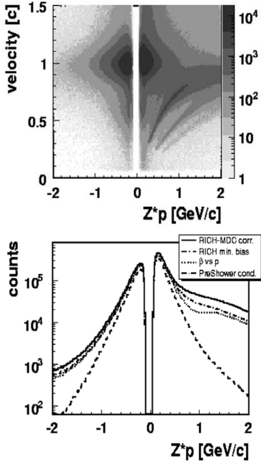
Fig. 41. The same as fig. 40 but for Ar + KCl collisions at 1.76 AGeV.
