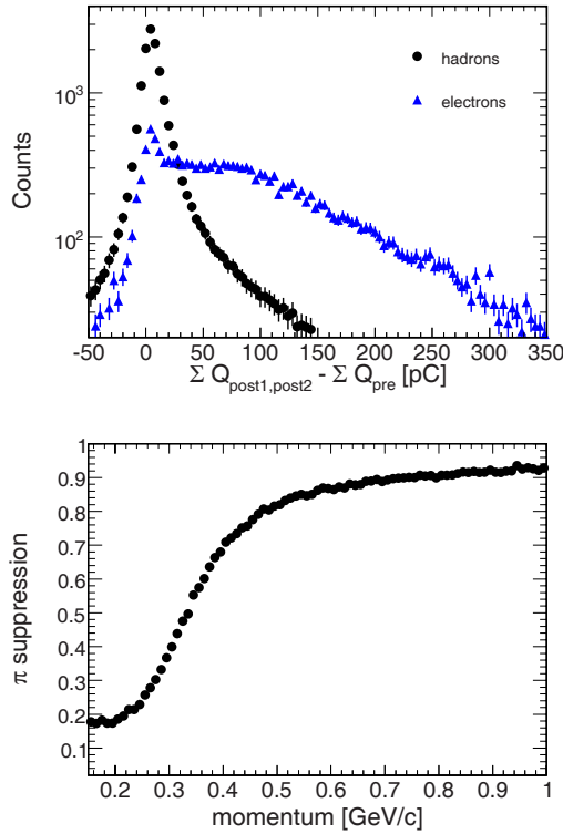
Fig. 23. Top: sum of charge \Sigma Q , over 3 \times 3 pads, measured on post1- and post2-chamber with subtracted charge measured in the pre-chamber. Electrons with momenta p \sim 0.5 GeV/ c (triangles) produce electromagnetic cascades in the Pb converters which results in a larger charge deposit compared to the one from hadrons, here \pi^- (dots). Bottom: pion suppression as a function of momentum: the fraction of pions rejected after the algorithm for lepton recognition (electromagnetic cascade) has been applied. Data are taken from 3.5 GeV p + p collisions.
