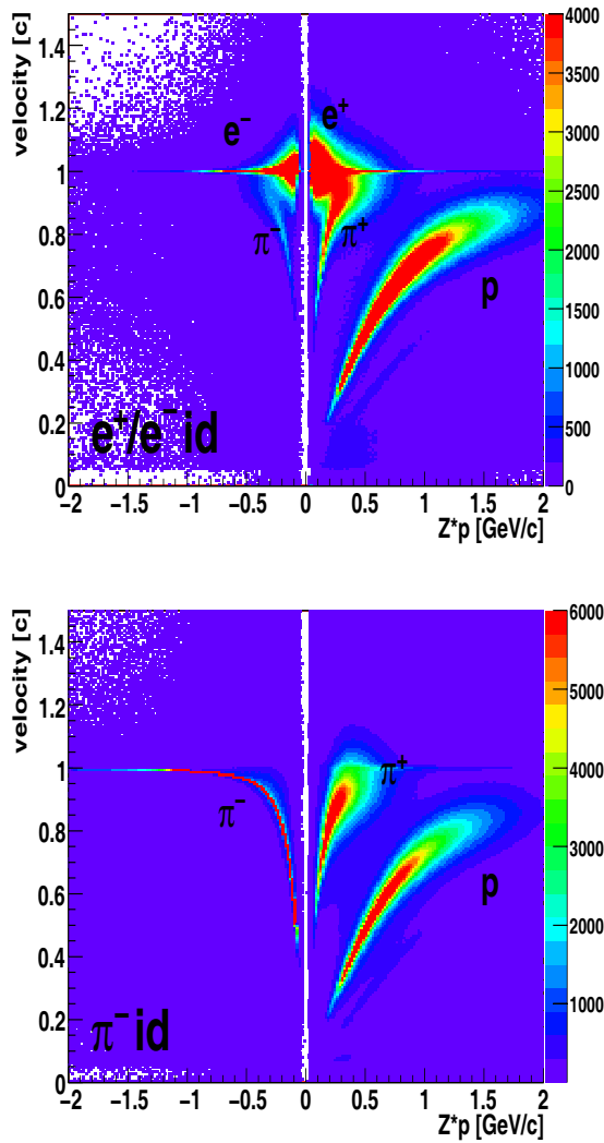
Fig. 19. Top: velocity versus Zp scatter plot for events from pp collisions at 2.2 GeV with an identified e^+/e^- . Bottom: the same but with an identified \pi^- .
