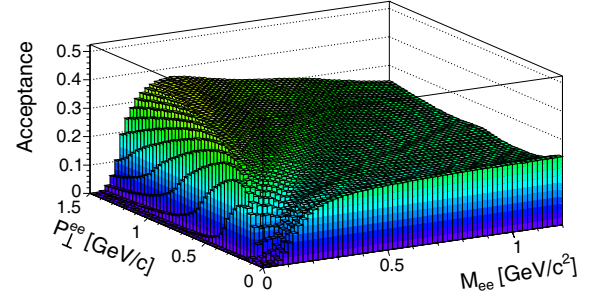
Fig. 42. Geometrical acceptance for e^+e^- pairs with opening angle \alpha_{e^+e^-} > 9^\circ as a function of pair mass and transverse momentum. The acceptance is averaged over a distribution in rapidity in the interval [0, 2] representative of the reactions at SIS energies.
