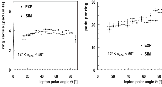
Fig. 9. Polar-angle distributions of Cherenkov ring properties for single electrons from open e^+e^- pairs produced in the reaction C + C at 1 AGeV (exp). Simulation results (sim) are shown for comparison. The error bars reflect the widths of the nearly Gaussian multiplicity distributions at each angle. Left: ring radius vs. lepton polar angle; right: mean number of pads within a region of 13 \times 13 pads around ring centers.
