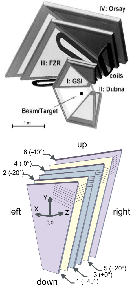
Fig. 10. Top: schematic layout of the HADES tracking system. Two sets of Mini-Drift Chambers (MDCs) with 24 wire planes per sector are placed in front and behind the magnetic field to measure particle momenta. Bottom: schematic view of the six anode wire frames inside a HADES MDC, representing the six stereo angles.
