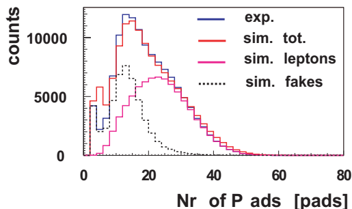
Figure 5.13: Distribution of the number of pads per ring, the experimental results are shown together with the simulations. The same number of events has been analyzed for the experimental and simulated data.
