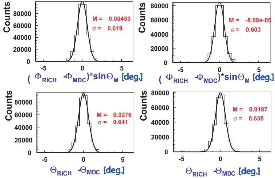
Figure A.6: The angular correlation (in deg.) extracted from the simulated data are shown. The reaction analyzed is C + C at 2 AGeV.
