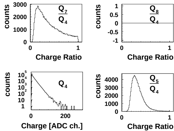
Figure 4.12: Experimental charge distribution for class 1 clusters. \frac{Q_7}{Q_4} and \frac{Q_5}{Q_4} are the ratios of the charge induced on the upper and right pads respectively divided by the charge induced on the central pad.
